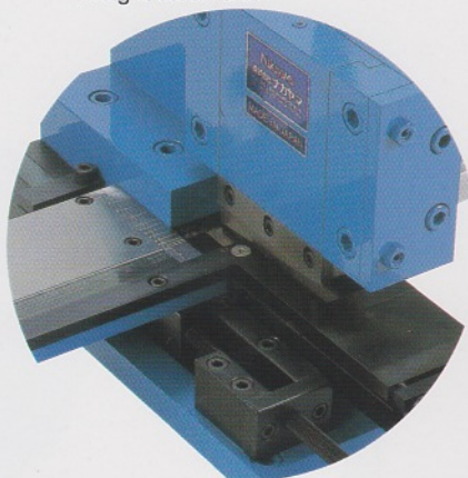
両切機切断面 Double Straight rule after being cut with our MODEL CT30BCD-S
